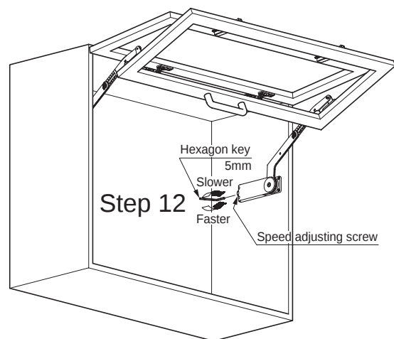
Fig. 11 Adjustment of door closing speed
