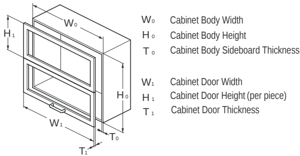
Fig.2 Cabinet illustration
