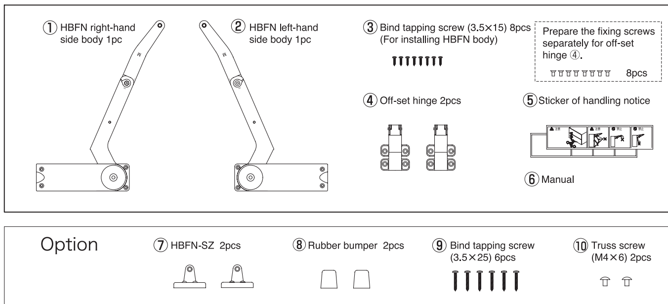
Fig. 1 Parts description
