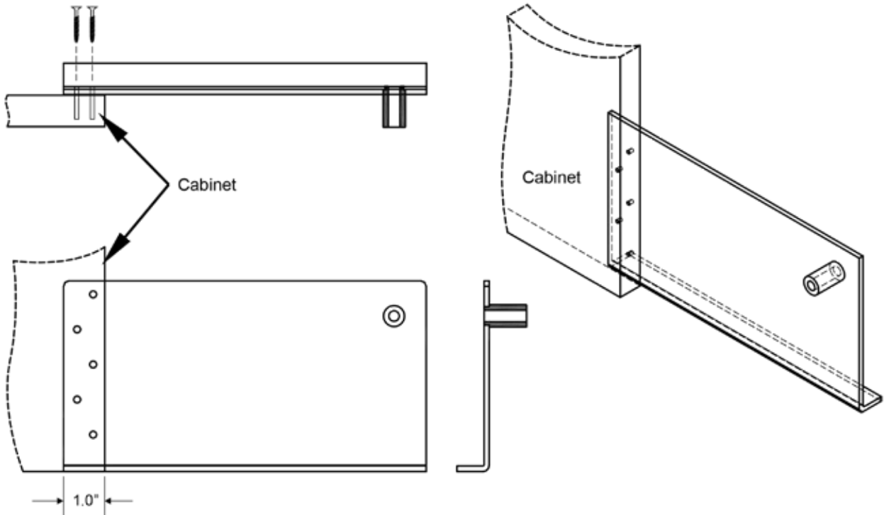
Drawing #3: Pivot Brackets
